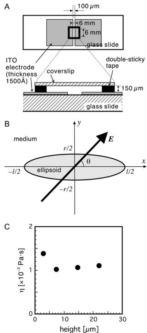
FIGURE 1 (A) Top and side views of the electroorientation chamber. Side view is vertically expanded to emphasize the structure. (B) Diagram illustrating a dielectric ellipsoid with its long axis x placed at angle \theta to the external field E . The z axis is perpendicular to the page. (C) Viscosity in the chamber is plotted as a function of the distance from the bottom of the electroorientation chamber. The rotational diffusion constant of microtubule D_r was measured from the mean square rotation angle of the microtubule \langle \theta^2 \rangle , and \eta was calculated from D_r = kT/\pi\eta^3 C_r = \langle \theta^2 \rangle/2t , where C_r is a form factor (Eq. 5) (55).
