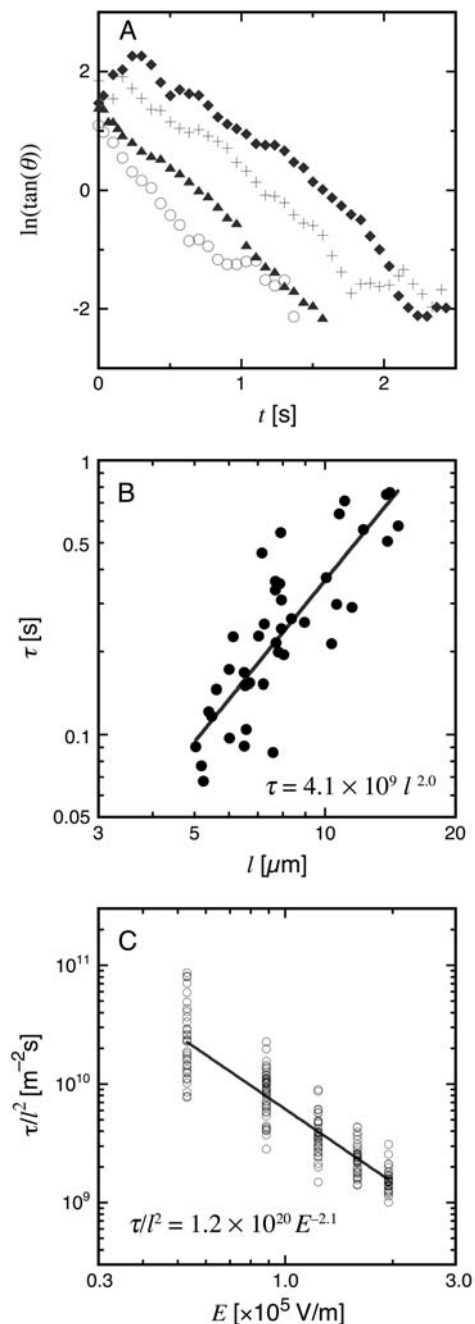
FIGURE 3 Quantitative analysis of microtubule electroorientation. (A) \ln(\tan(\theta)) plotted against time. Since the taxol-stabilized microtubule is rigid enough, \theta can be uniquely determined at each time instant (see Gittes et al. (56)). Four representative examples for microtubules with lengths of 8–12 \mu\text{m} are shown. E = 1.2 \times 10^5 V/m, frequency 1 MHz. (B) Electroorientation time constant \tau plotted as a function of the microtubule length l . \tau is proportional to the square of the filament length (line represents the best fit: \tau = 4.1 \times 10^9 l^{2.0} ). (C) Time constant normalized for the square of microtubule length, \tau/l^2 , plotted as a function of the field strength E . Line represents the best fit: \tau/l^2 = 1.2 \times 10^{20} E^{-2.1} .
