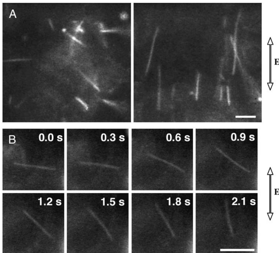
FIGURE 2 Orientation of microtubules at E = 9 \times 10^4 V/m, frequency 1 MHz. (A, Left ) Orientation of microtubules is random in the absence of the electric field. ( Right ) Upon application of the electric field, the microtubules are oriented parallel to the direction of the field line. (B) Sequential images of a single microtubule after the onset of the electric field taken at intervals of 0.3 s. Arrows indicate the direction of the applied electric field. Scale bar, 10 \mu\text{m} .
